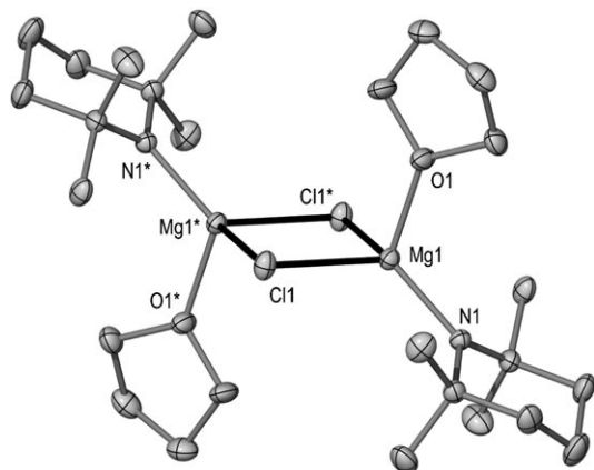
Figure 1. Molecular structure of 1 with hydrogen atoms and disordered toluene of crystallization omitted for clarity.
