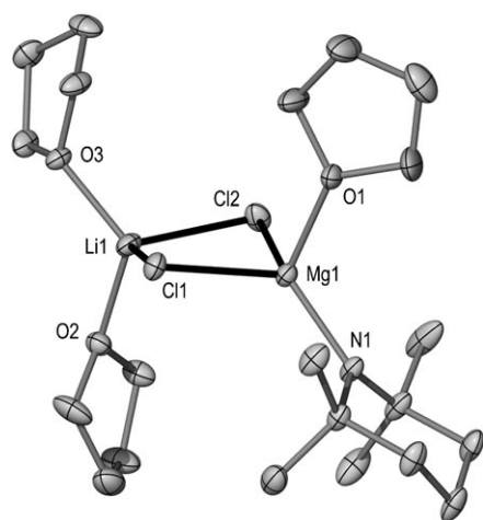
Figure 2. Molecular structure of 2 with hydrogen atoms omitted for clarity.
